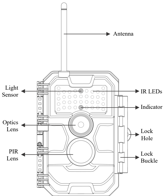
Figure 1: Front View
